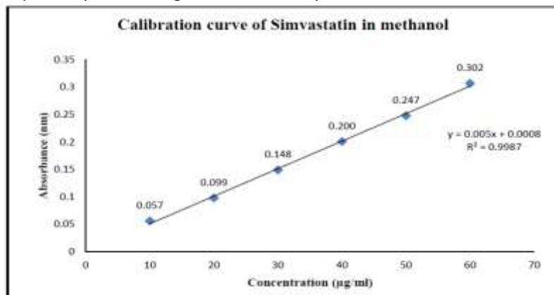
Figure 2: Calibration curve of Simvastatin in methanol
