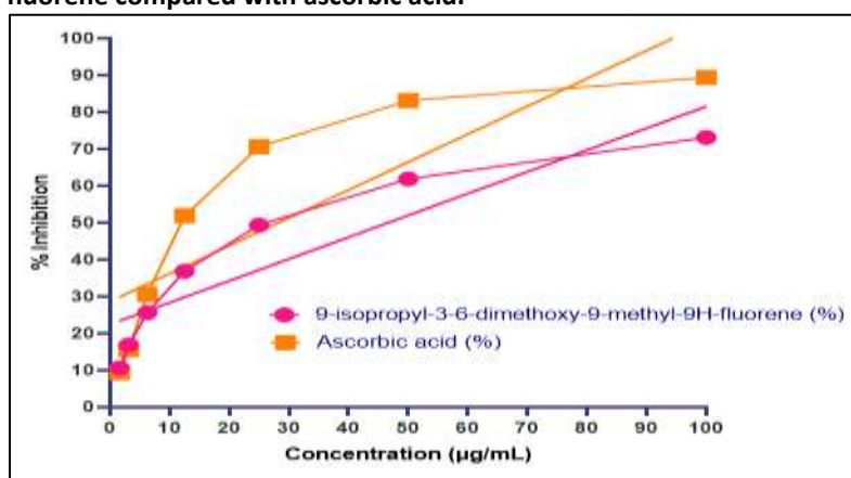
Figure 1: Concentration-dependent DPPH radical-scavenging activity of 9-isopropyl-3,6-dimethoxy-9-methyl-9H-fluorene compared with ascorbic acid.
