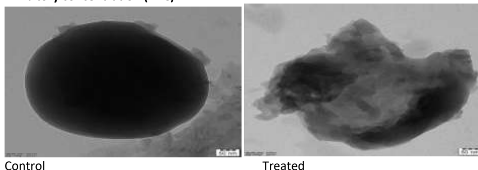
Figure 3: HR-TEM images of Staphylococcus aureus showing the untreated control cell and the morphological alterations observed following treatment with 9-isopropyl-3,6-dimethoxy-9-methyl-9H-fluorene at its minimum inhibitory concentration (MIC).
